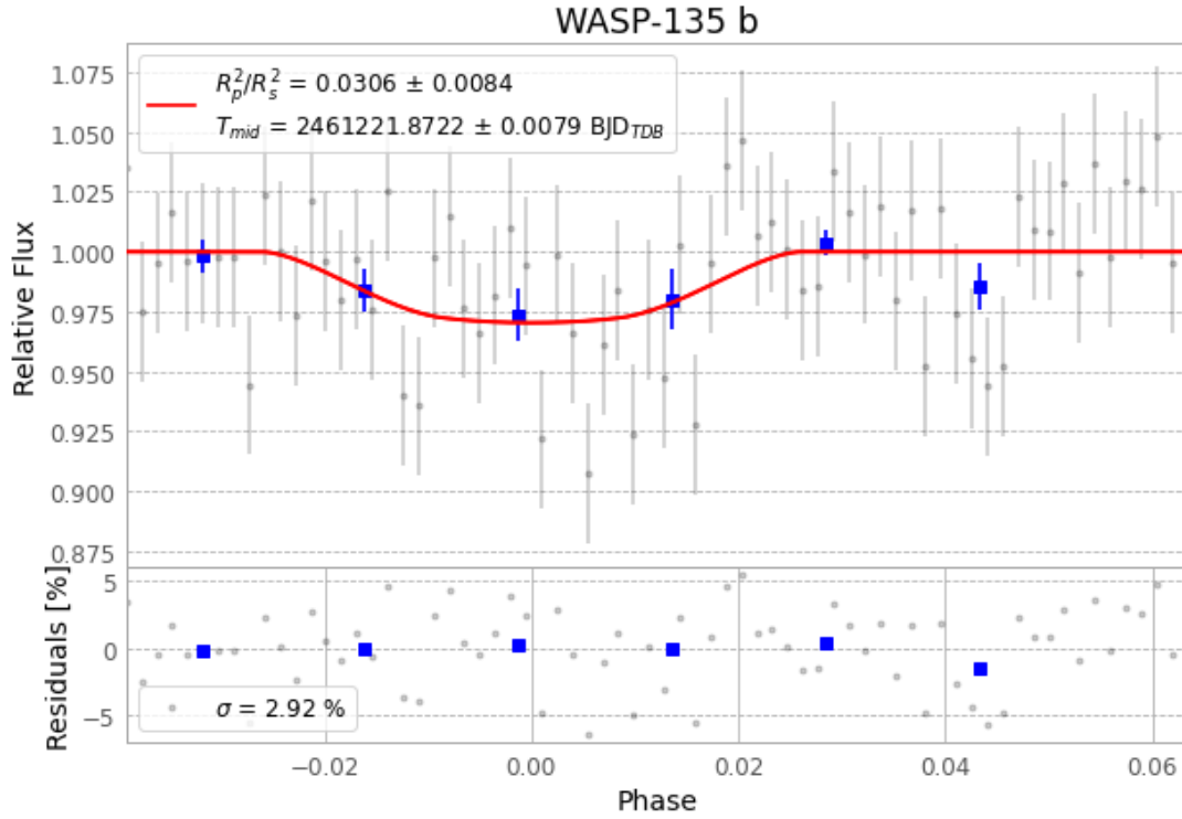
Figure 1 — FinalLightCurve_WASP-135 b_2026-06-30.png (SHA-256 0b91ce318af1ed99...)
