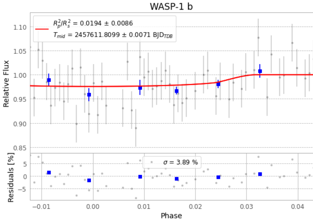
Figure 1 — FinalLightCurve_WASP-1 b_2016-08-10.png (SHA-256 1acaa0b0af6657bf...)
