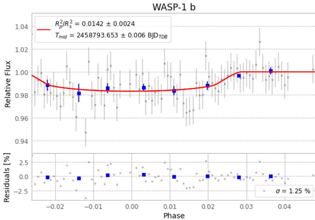
Figure 1 — FinalLightCurve_WASP-1 b_2019-11-05.png (SHA-256 2be58eff8052b98e...)
