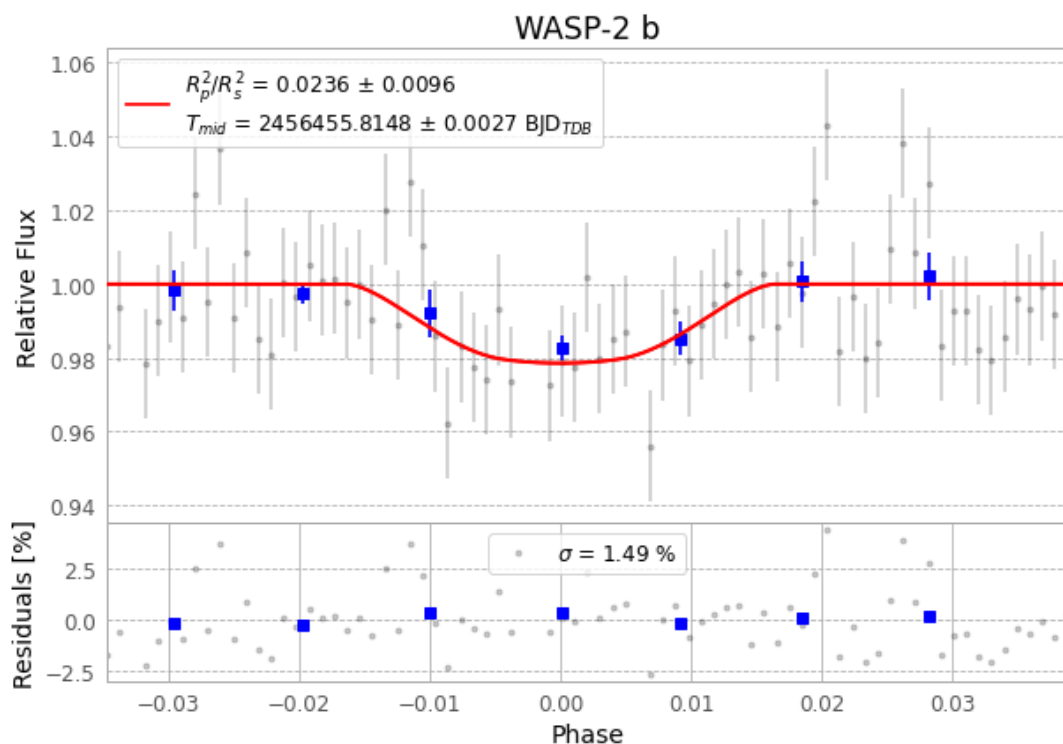
Figure 1 — FinalLightCurve_WASP-2 b_2013-06-11.png (SHA-256 d82efe683fb8e20f...)
