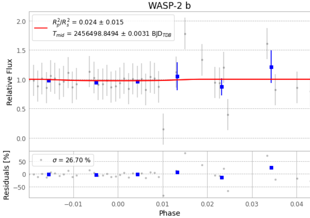
Figure 1 — FinalLightCurve_WASP-2 b_2013-07-25.png (SHA-256 45ea4651d4db10b8...)
