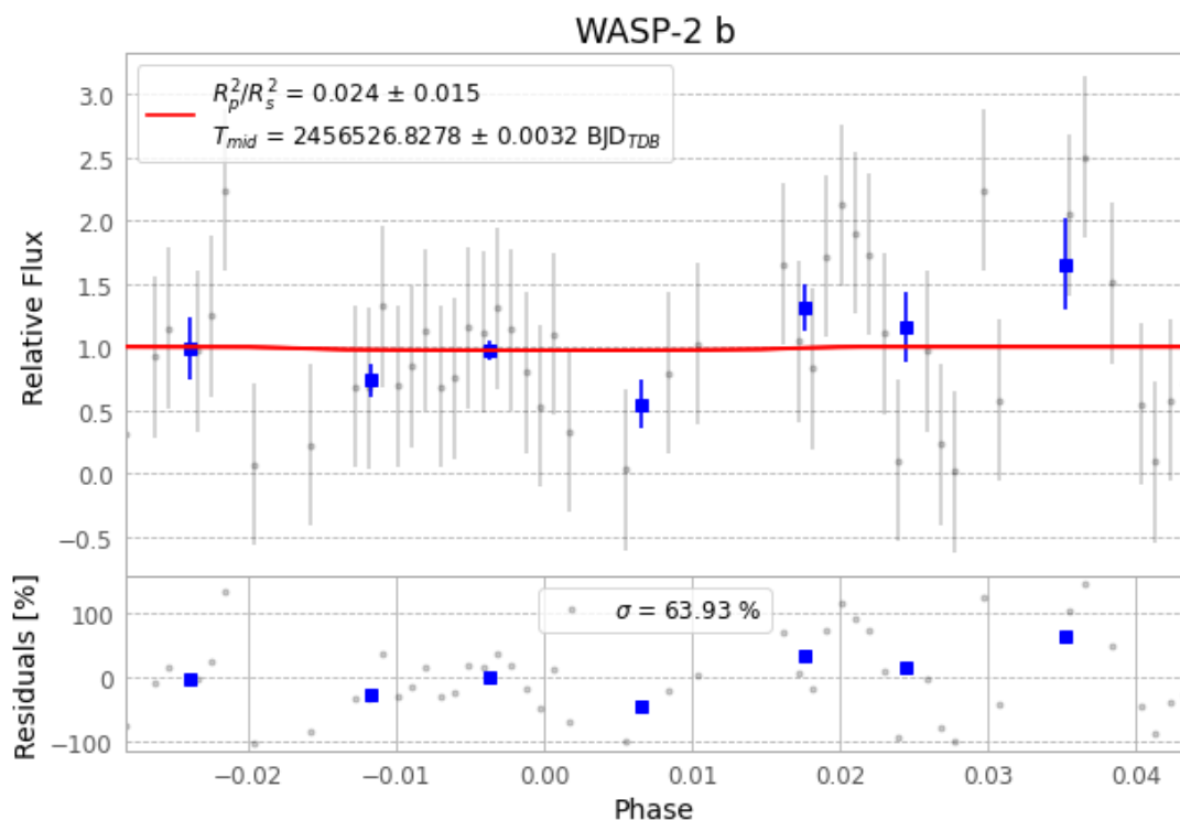
Figure 1 — FinalLightCurve_WASP-2 b_2013-08-21.png (SHA-256 3a638f0b4271260d...)
