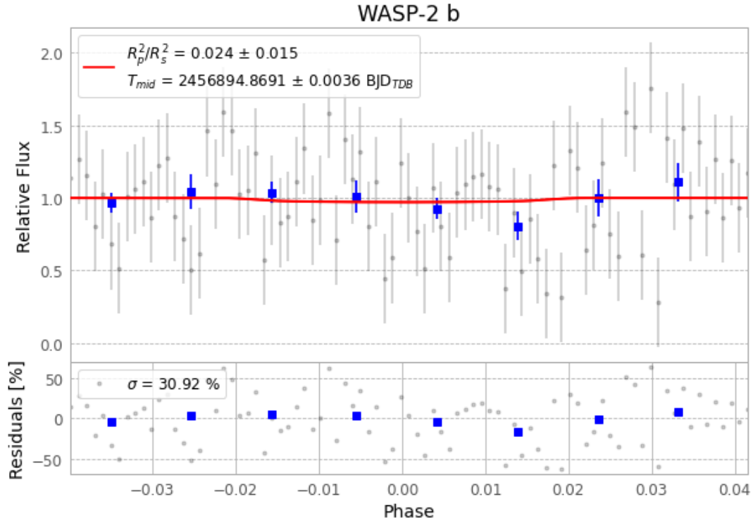
Figure 1 — FinalLightCurve_WASP-2 b_2014-08-24.png (SHA-256 b34360e608dedf11...)
