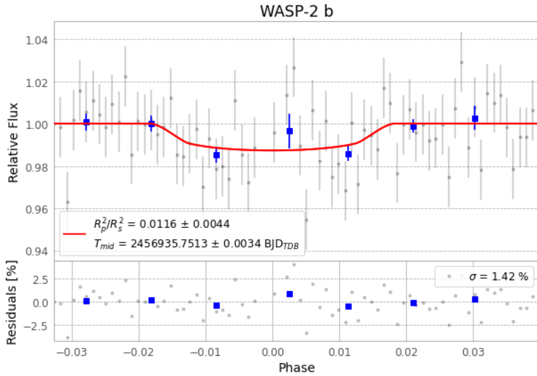
Figure 1 — FinalLightCurve_WASP-2 b_2014-10-04.png (SHA-256 f814f1122c3b9211...)
