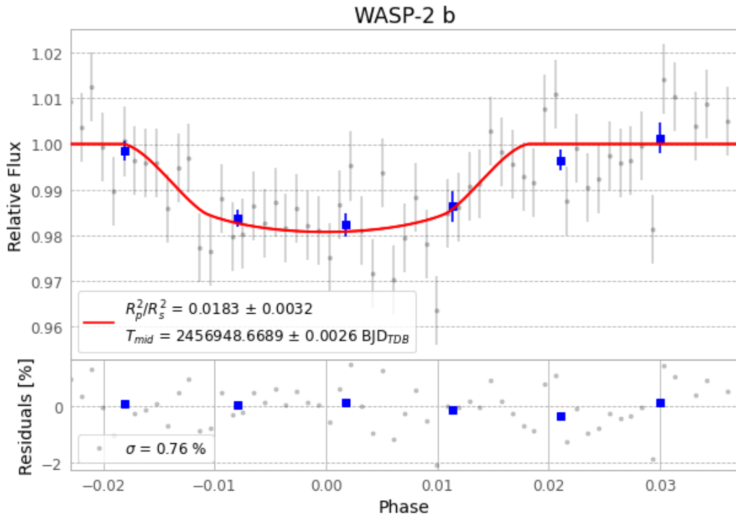
Figure 1 — FinalLightCurve_WASP-2 b_2014-10-17.png (SHA-256 6fc4b2edd19cb655...)
