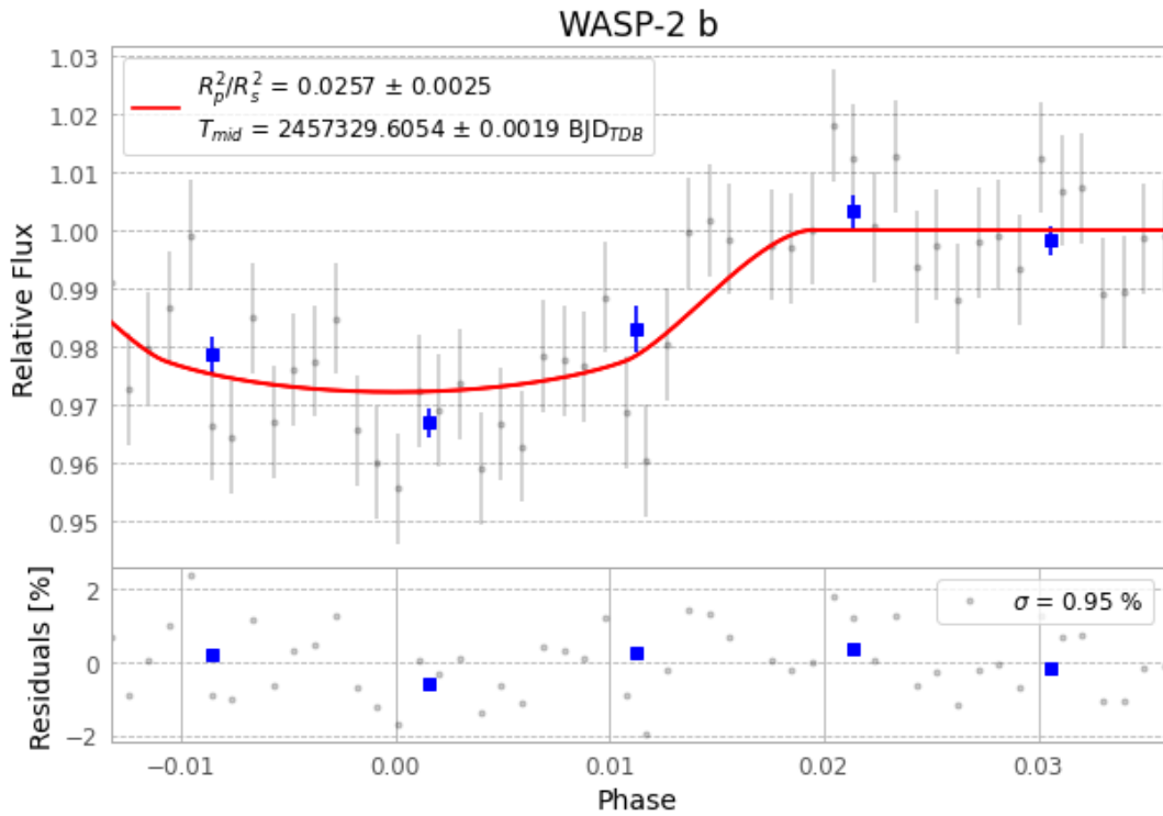
Figure 1 — FinalLightCurve_WASP-2 b_2015-11-02.png (SHA-256 f20c582915b92fa5...)
