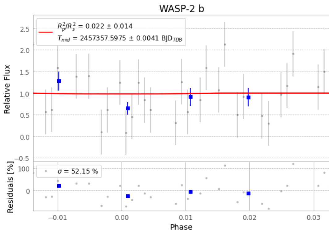
Figure 1 — FinalLightCurve_WASP-2 b_2015-11-30.png (SHA-256 7f4d5ee6a8405295...)
