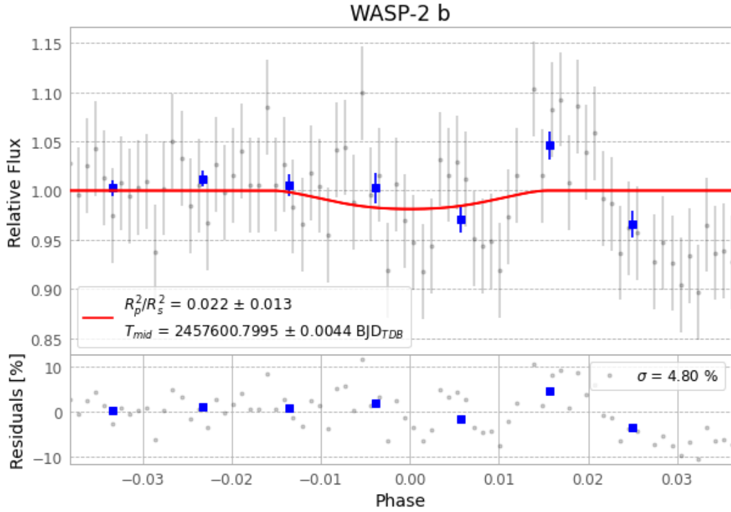
Figure 1 — FinalLightCurve_WASP-2 b_2016-07-30.png (SHA-256 2511ab54f728bf1e...)
