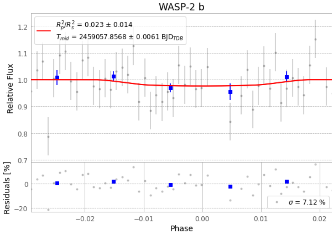
Figure 1 — FinalLightCurve_WASP-2 b_2020-07-26.png (SHA-256 7175f58a0c89cb92...)
