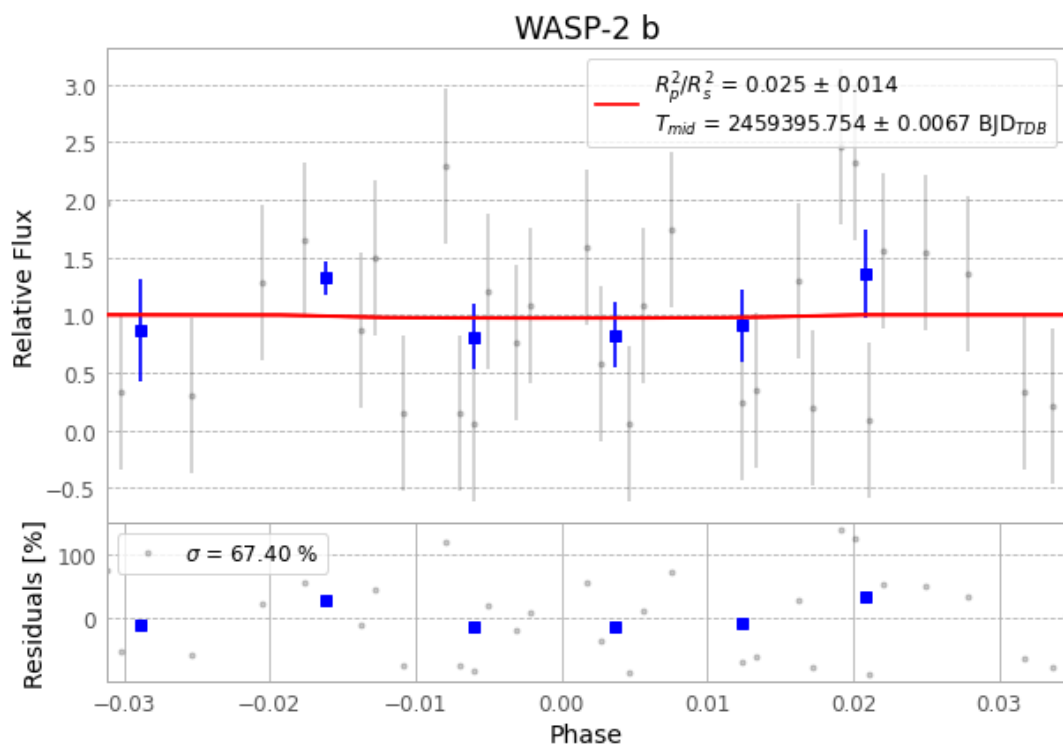
Figure 1 — FinalLightCurve_WASP-2 b_2021-06-29.png (SHA-256 0a1c6af028a677e1...)
