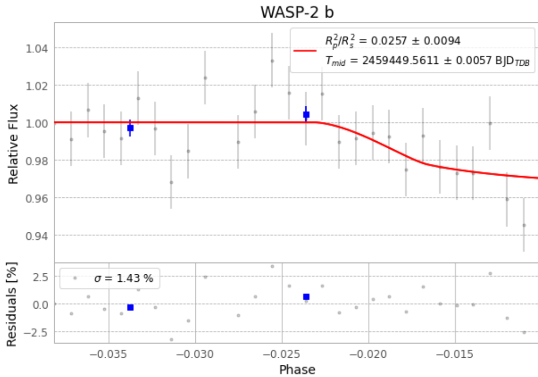
Figure 1 — FinalLightCurve_WASP-2 b_2021-08-24.png (SHA-256 f9fbbc082437b77e...)
