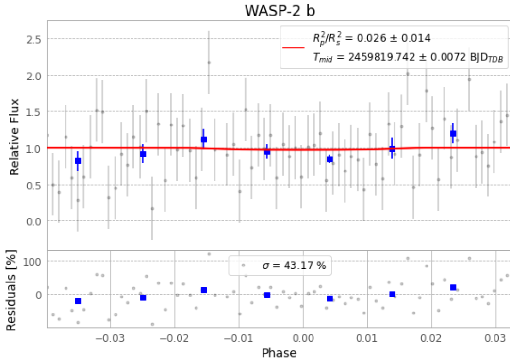
Figure 1 — FinalLightCurve_WASP-2 b_2022-08-27.png (SHA-256 0ffac0f1e1a9e9a9...)
