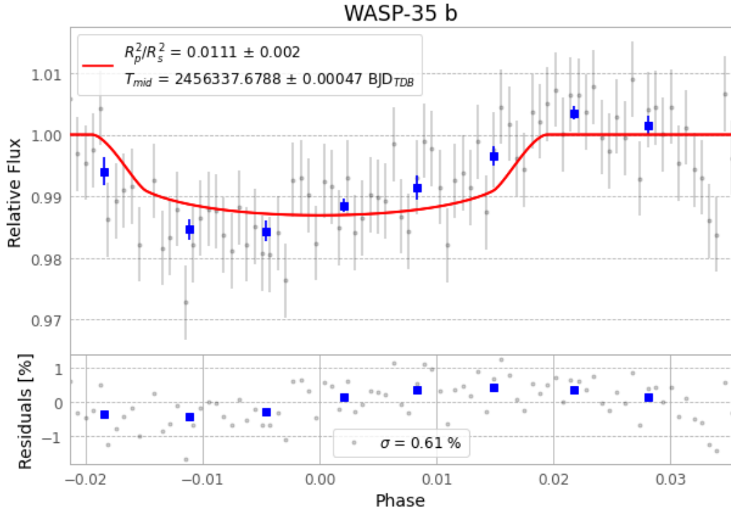
Figure 1 — FinalLightCurve_WASP-35 b_2013-02-13.png (SHA-256 a48e1cef150ea6a4...)
