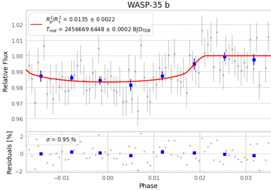
Figure 1 — FinalLightCurve_WASP-35 b_2014-01-11.png (SHA-256 d36d1993e8ec8aa2...)
