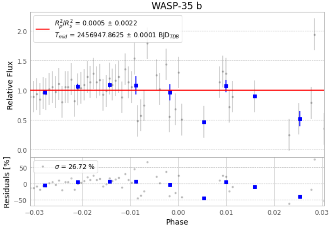
Figure 1 — FinalLightCurve_WASP-35 b_2014-10-16.png (SHA-256 0b4926f365a5ef7d...)
