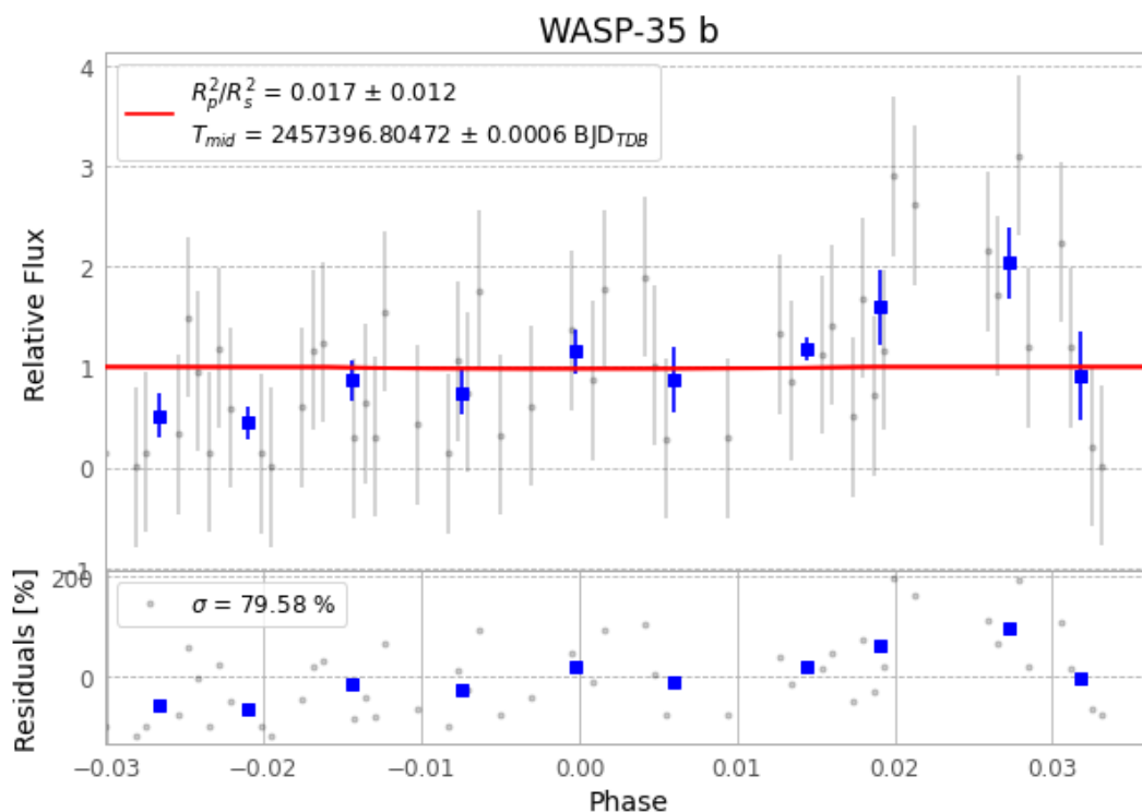
Figure 1 — FinalLightCurve_WASP-35 b_2016-01-08.png (SHA-256 ac6885641c3094d6...)
