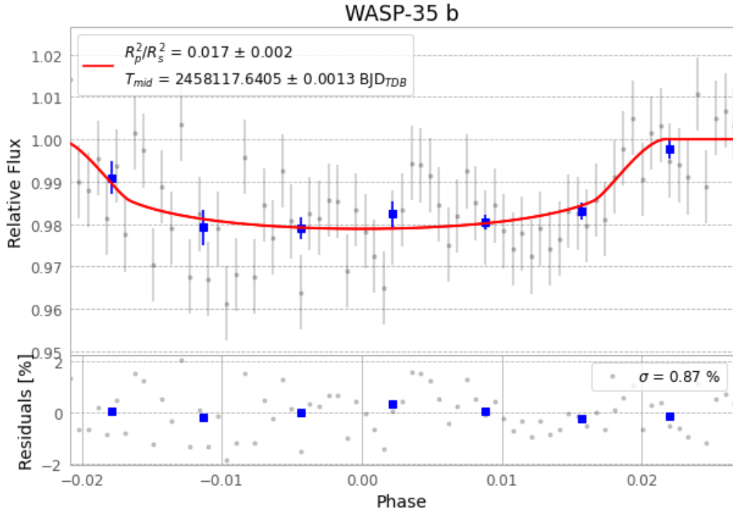
Figure 1 — FinalLightCurve_WASP-35 b_2017-12-29.png (SHA-256 8d8cd8c27b18fa9c...)
