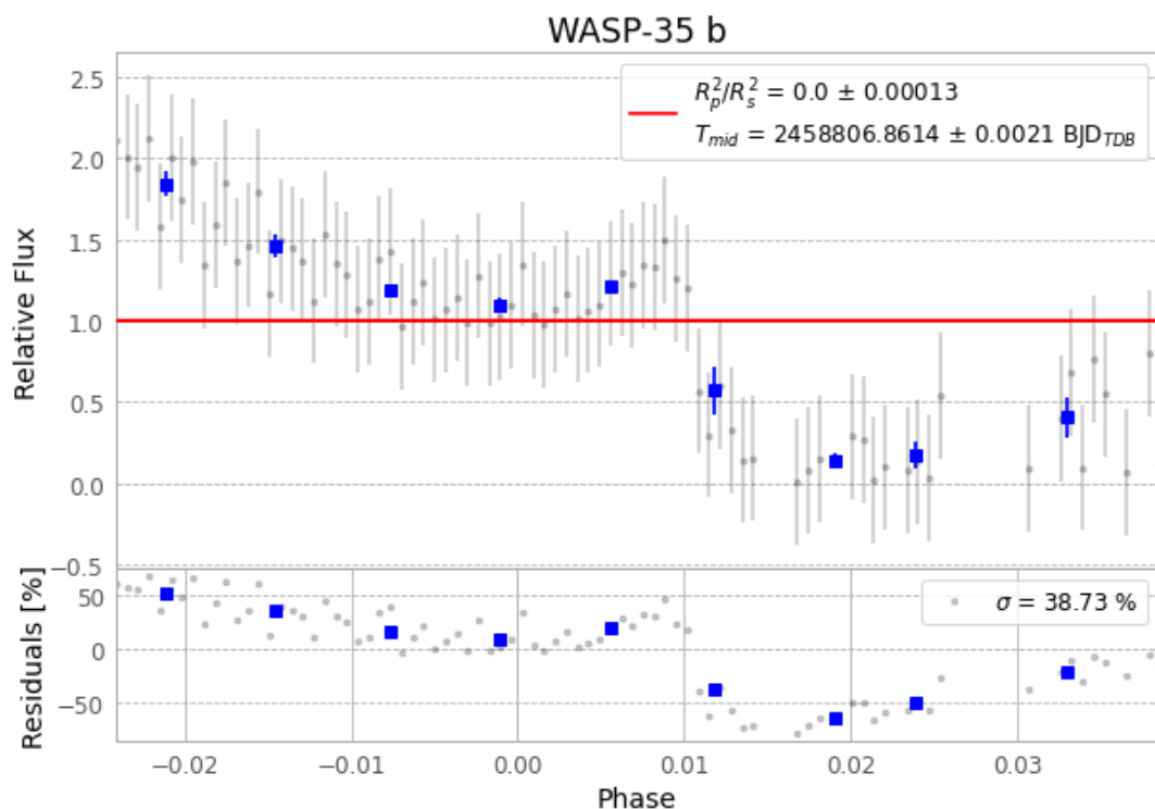
Figure 1 — FinalLightCurve_WASP-35 b_2019-11-18.png (SHA-256 baac2c950231d350...)
