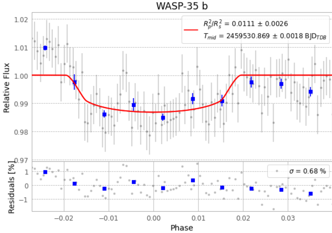
Figure 1 — FinalLightCurve_WASP-35 b_2021-11-11.png (SHA-256 d43e5d3bf3cdf05...)
