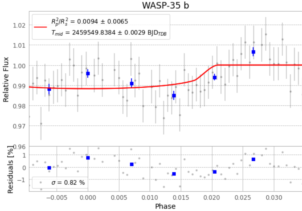
Figure 1 — FinalLightCurve_WASP-35 b_2021-12-01.png (SHA-256 7138c1e33964f815...)
