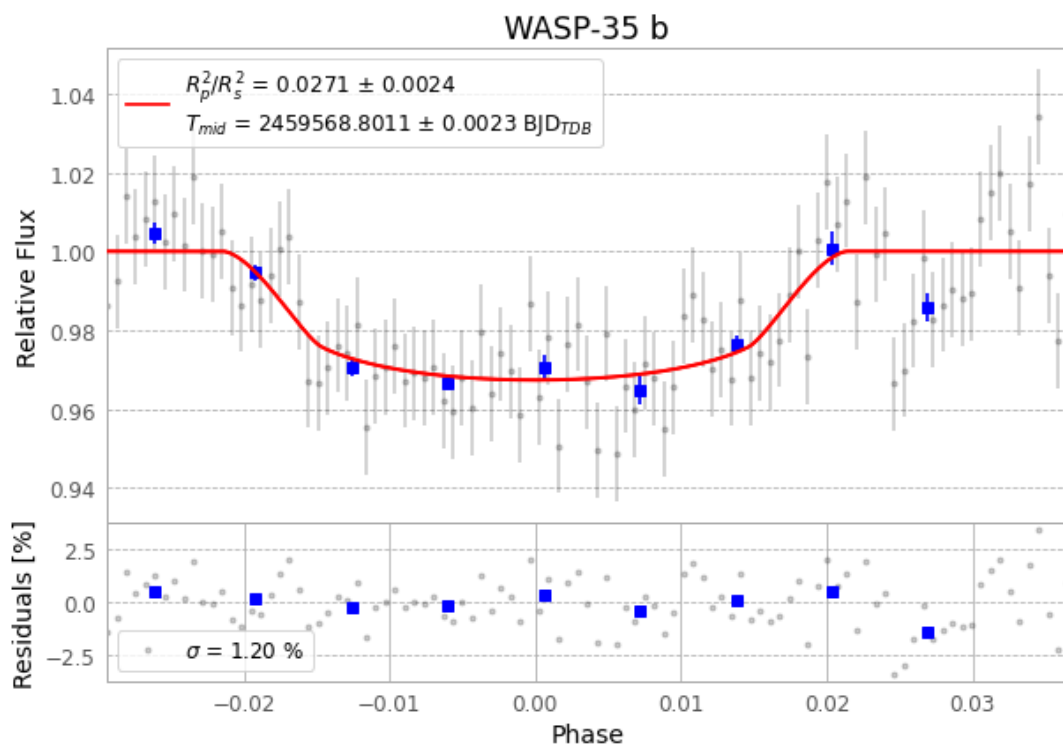
Figure 1 — FinalLightCurve_WASP-35 b_2021-12-19.png (SHA-256 f376f40be6ea36e9...)
