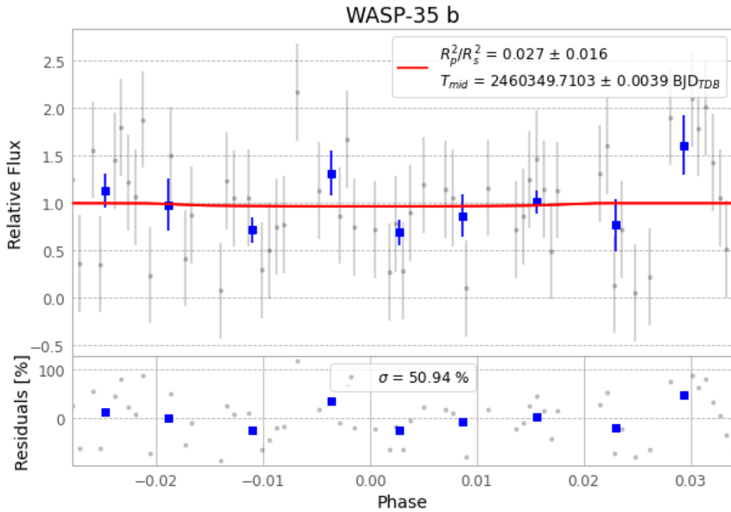
Figure 1 — FinalLightCurve_WASP-35 b_2024-02-08.png (SHA-256 2955b6c824aa7a80...)
