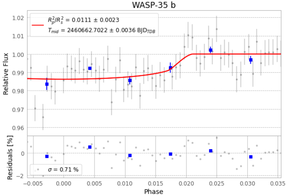
Figure 1 — FinalLightCurve_WASP-35 b_2024-12-17.png (SHA-256 592b86f4eea17c96...)
