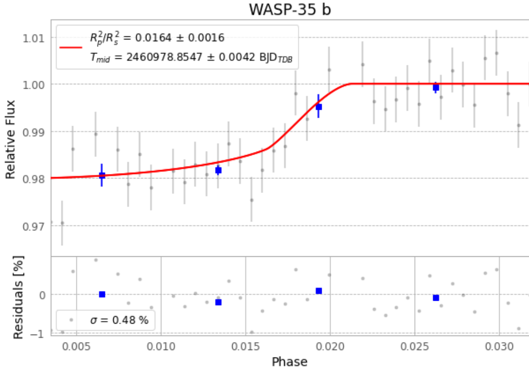
Figure 1 — FinalLightCurve_WASP-35 b_2025-10-30.png (SHA-256 be63eded15d001d6...)
