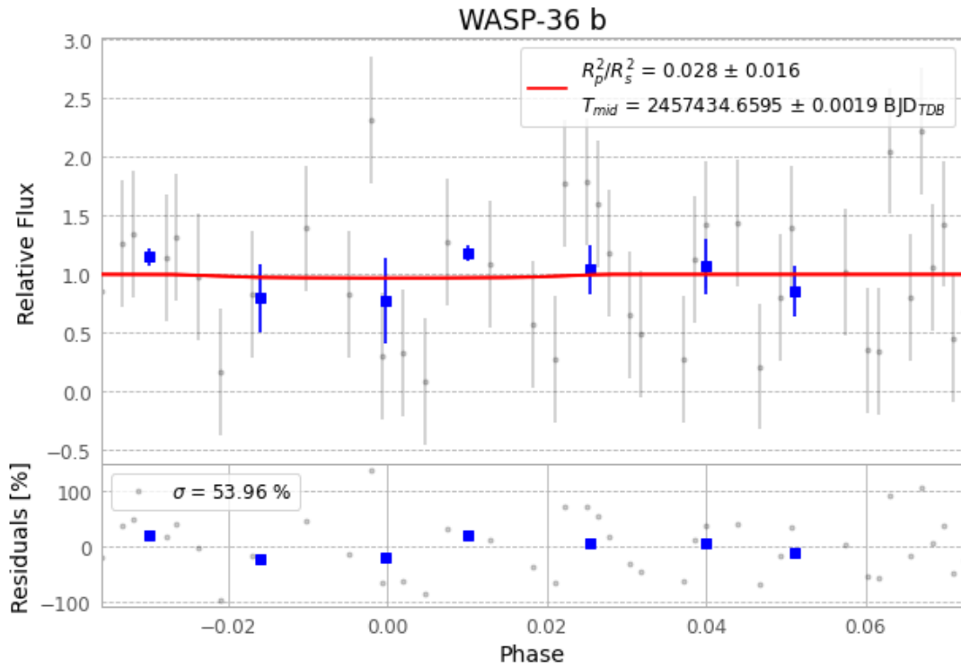
Figure 1 — FinalLightCurve_WASP-36 b_2016-02-15.png (SHA-256 c0a6432317f4ea84...)
