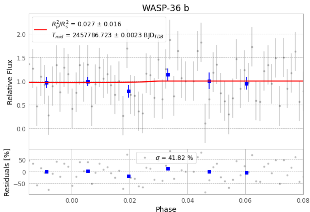
Figure 1 — FinalLightCurve_WASP-36 b_2017-02-01.png (SHA-256 6d927f77064ee080...)
