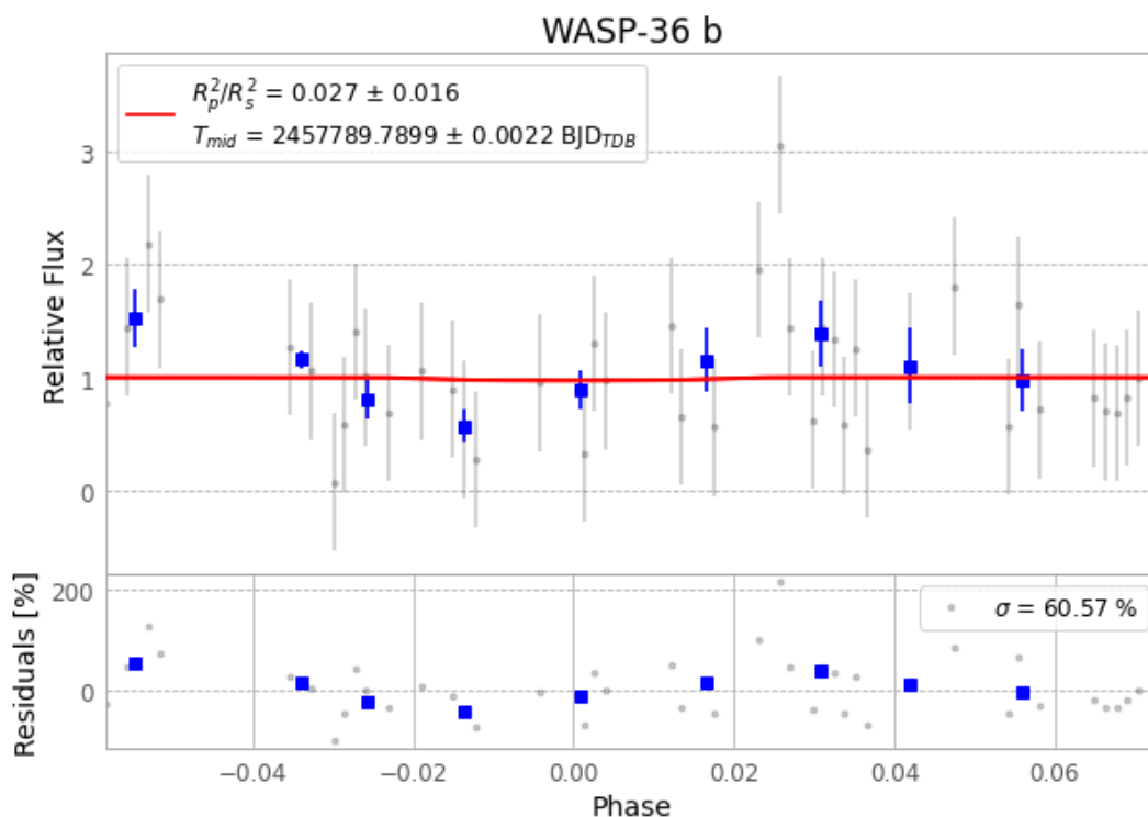
Figure 1 — FinalLightCurve_WASP-36 b_2017-02-04.png (SHA-256 21b63b587a910afe...)
