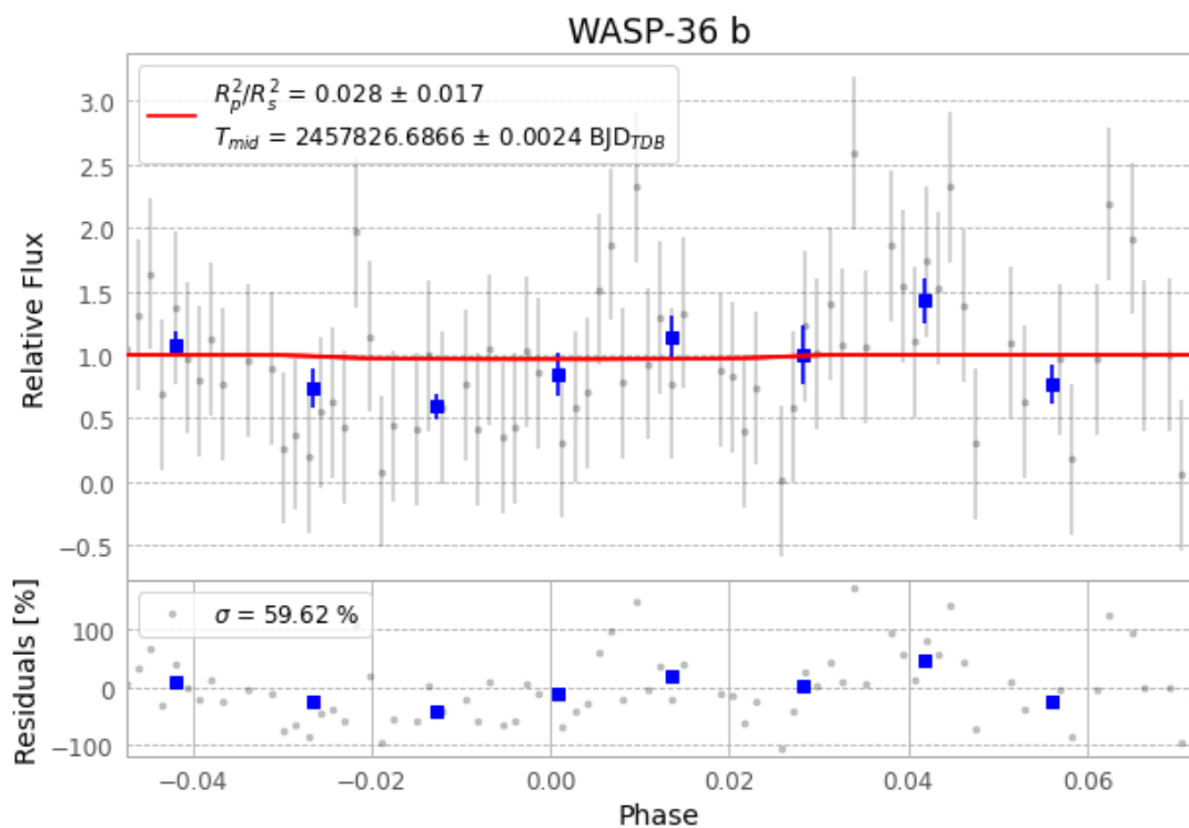
Figure 1 — FinalLightCurve_WASP-36 b_2017-03-13.png (SHA-256 e57208ef67367cad...)
