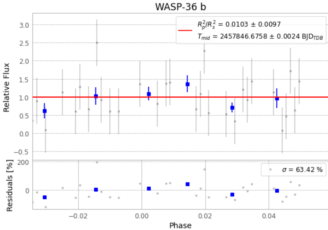
Figure 1 — FinalLightCurve_WASP-36 b_2017-04-02.png (SHA-256 109b95a22fba31f9...)
