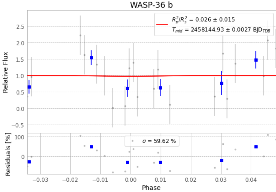
Figure 1 — FinalLightCurve_WASP-36 b_2018-01-26.png (SHA-256 60210e7b6b909cb0...)
