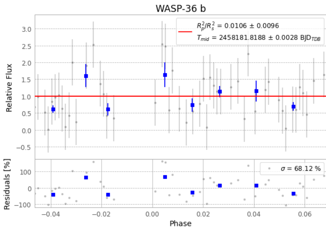
Figure 1 — FinalLightCurve_WASP-36 b_2018-03-03.png (SHA-256 687714f0e24ff8ca...)
