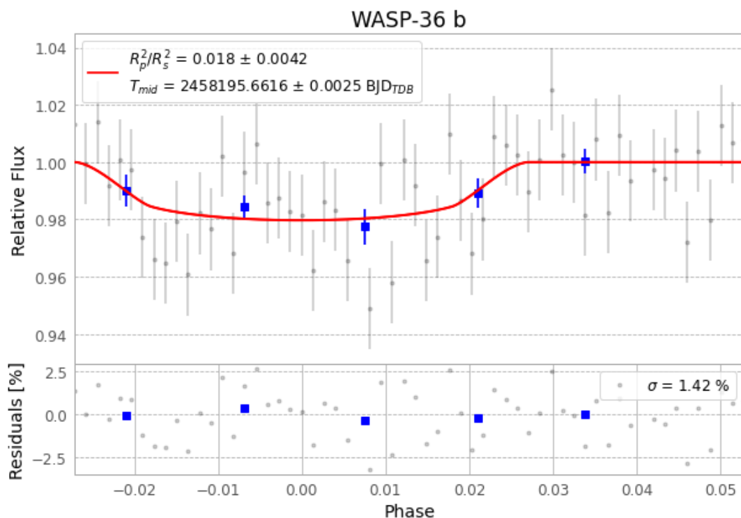
Figure 1 — FinalLightCurve_WASP-36 b_2018-03-17.png (SHA-256 99dae20ec0fcfb8b...)
