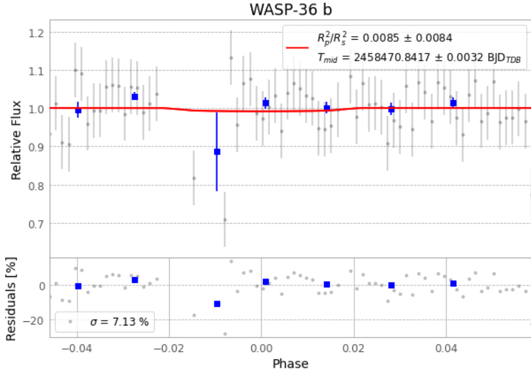
Figure 1 — FinalLightCurve_WASP-36 b_2018-12-17.png (SHA-256 3f06b74abf14a291...)
