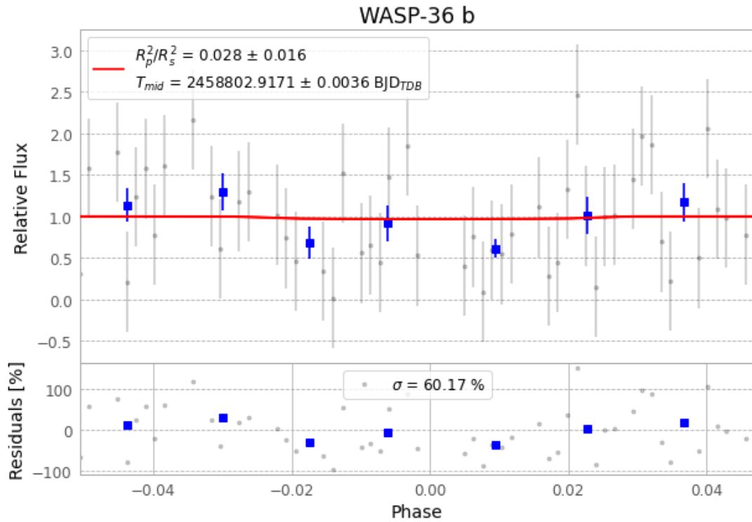
Figure 1 — FinalLightCurve_WASP-36 b_2019-11-15.png (SHA-256 1298a104e7e613f8...)
