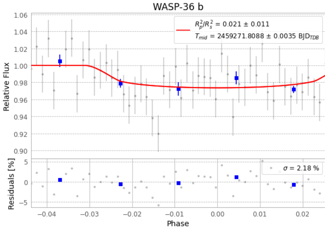
Figure 1 — FinalLightCurve_WASP-36 b_2021-02-25.png (SHA-256 ab2a345c82349dbd...)
