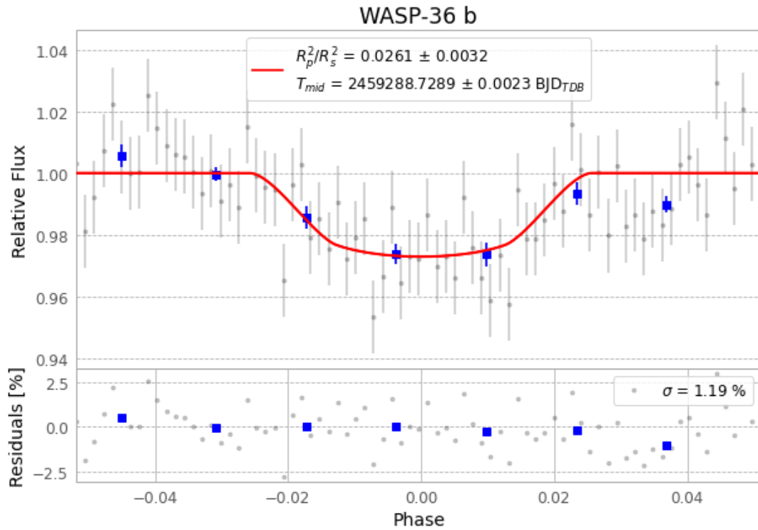
Figure 1 — FinalLightCurve_WASP-36 b_2021-03-14.png (SHA-256 23ce7c0e6cd843e6...)
