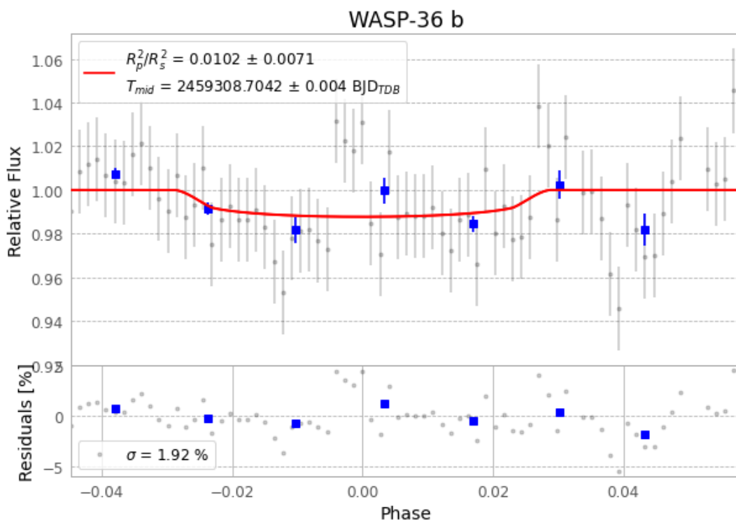
Figure 1 — FinalLightCurve_WASP-36 b_2021-04-03.png (SHA-256 18cdc398f393612e...)
