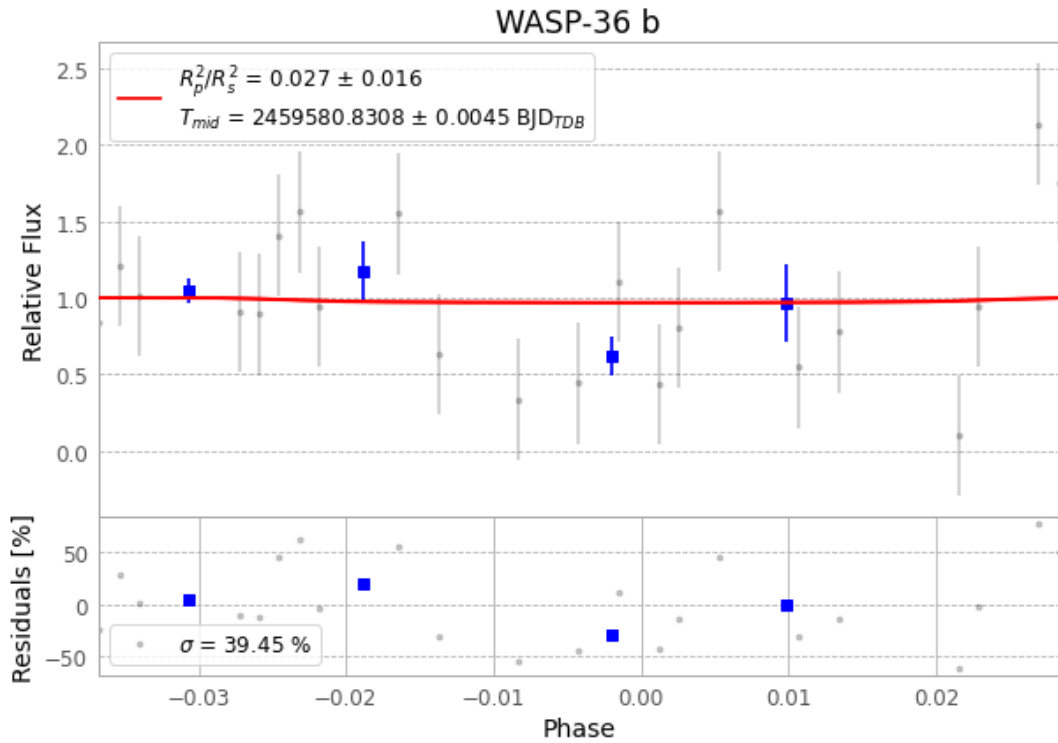
Figure 1 — FinalLightCurve_WASP-36 b_2021-12-31.png (SHA-256 5d7bcfac993ce5ed...)
