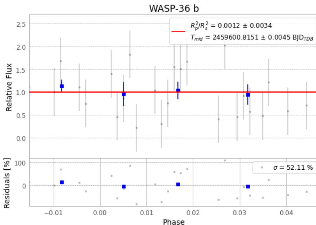
Figure 1 — FinalLightCurve_WASP-36 b_2022-01-20.png (SHA-256 66038e042194bf94...)
