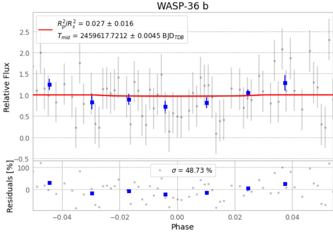
Figure 1 — FinalLightCurve_WASP-36 b_2022-02-06.png (SHA-256 d93752b2af06d9fa...)
