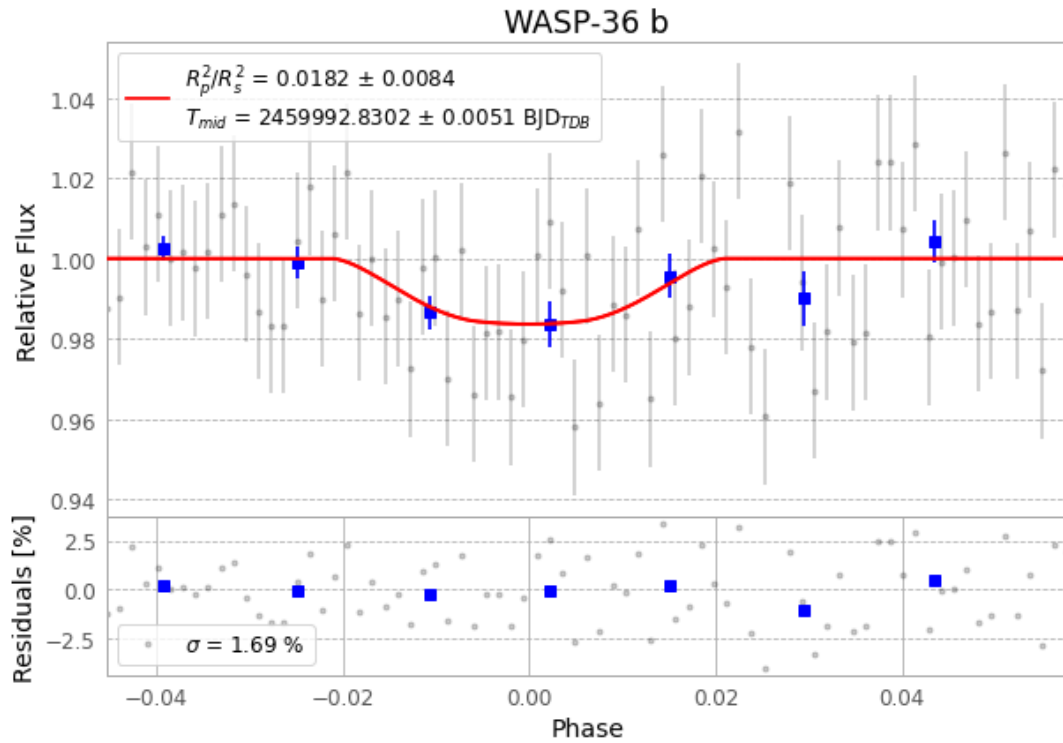
Figure 1 — FinalLightCurve_WASP-36 b_2023-02-16.png (SHA-256 2550da0af8087b65...)
