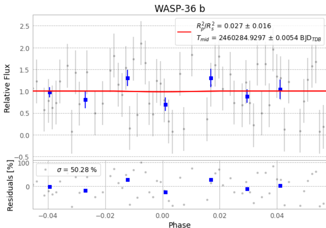
Figure 1 — FinalLightCurve_WASP-36 b_2023-12-06.png (SHA-256 1269bd029f7abee0...)
