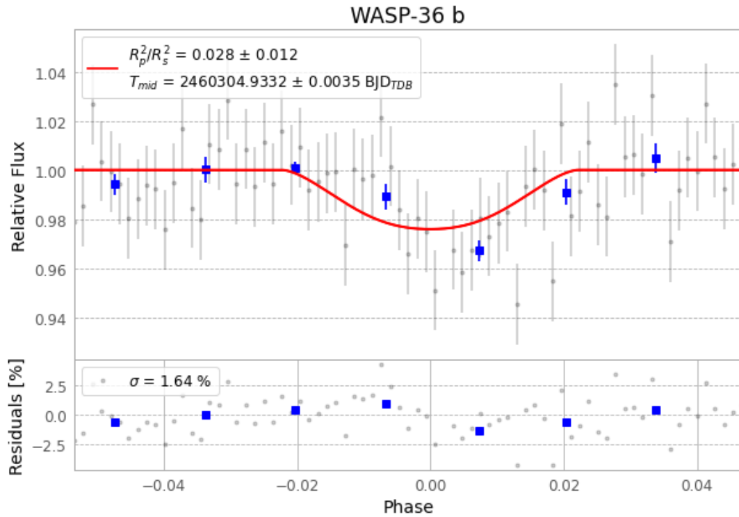
Figure 1 — FinalLightCurve_WASP-36 b_2023-12-26.png (SHA-256 519037b0ade6fb7f...)
