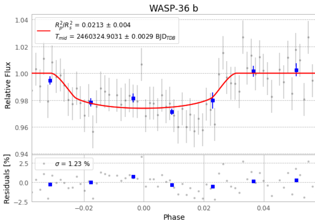
Figure 1 — FinalLightCurve_WASP-36 b_2024-01-15.png (SHA-256 b7ec8c263daf6ea3...)
