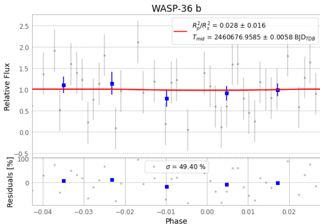
Figure 1 — FinalLightCurve_WASP-36 b_2025-01-01.png (SHA-256 02ae5d2d07d5846b...)
