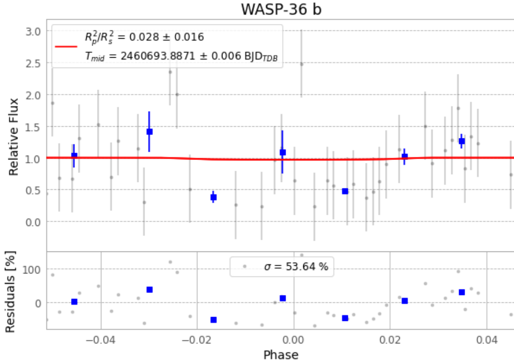
Figure 1 — FinalLightCurve_WASP-36 b_2025-01-18.png (SHA-256 dcd6b9e6c08f148a...)
